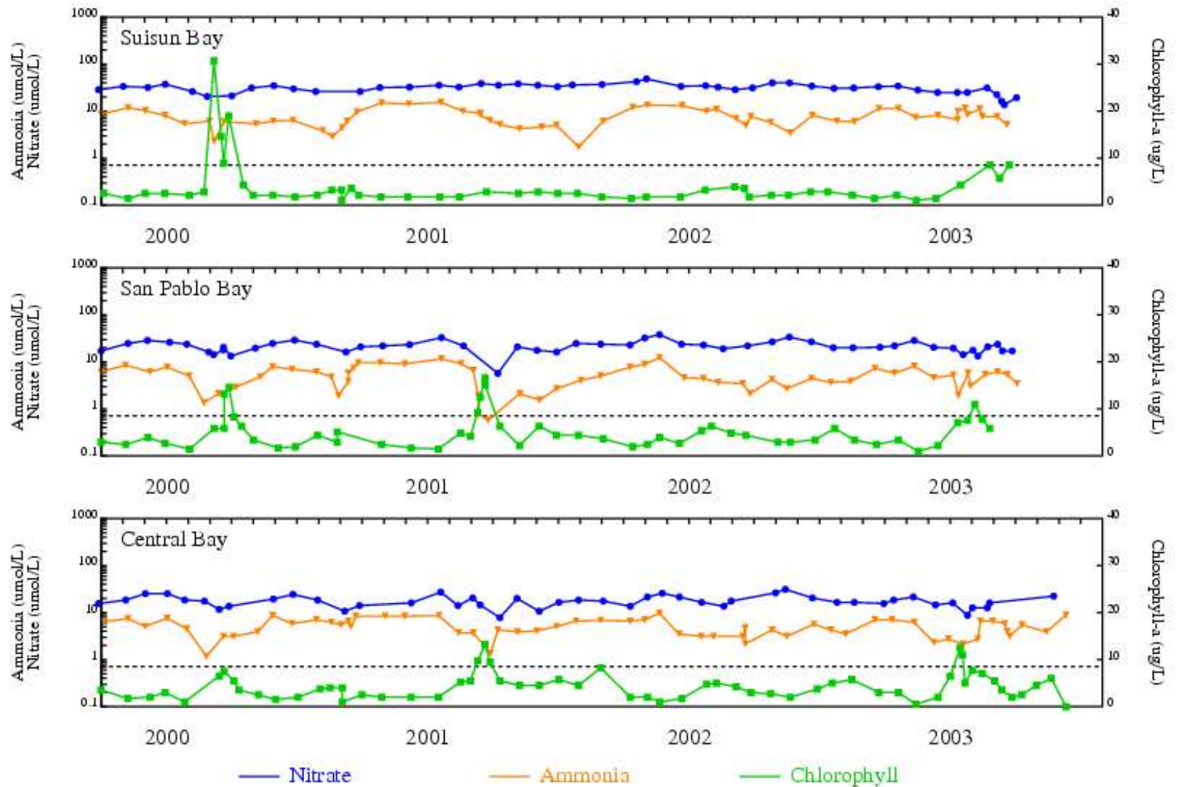
Ammonia, Nitrate and Chlorophyll-a in the San Francisco Delta Source: Dugdale, 2007
